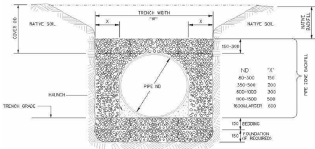
Figure 5: Minimum Trench Width
