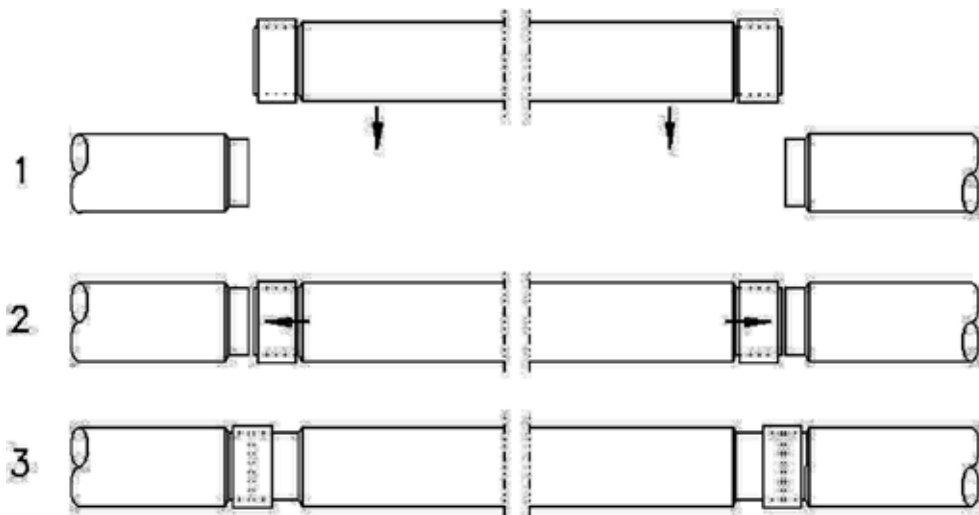
Figure 14: Pipeline closure
