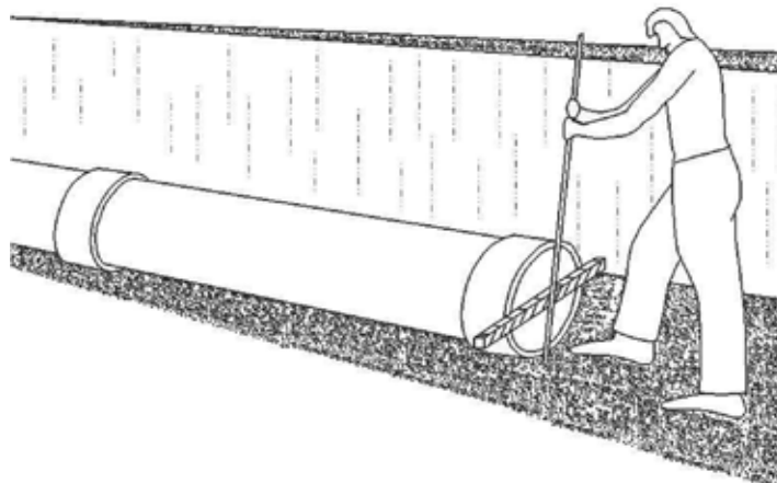
Figure 10: Mounting the coupling for DN \square 350 mm
