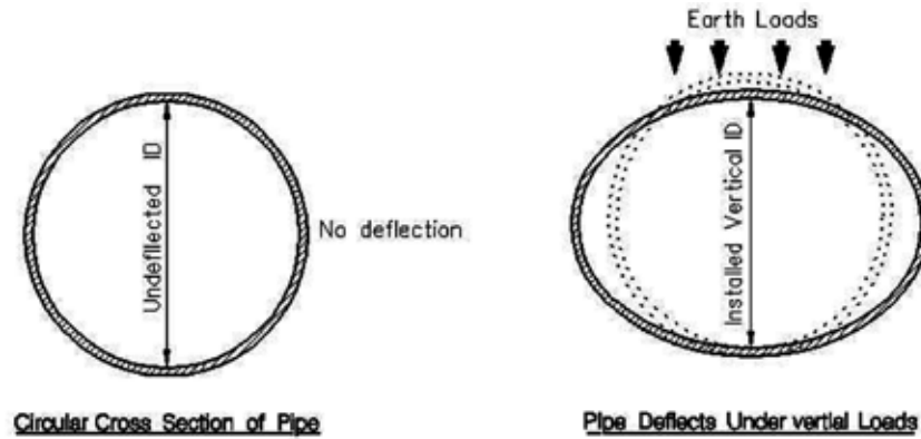
Figure 17: Pipe deflection
