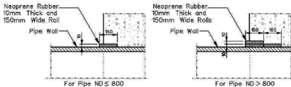
Figure 15: Rubber wrapping
