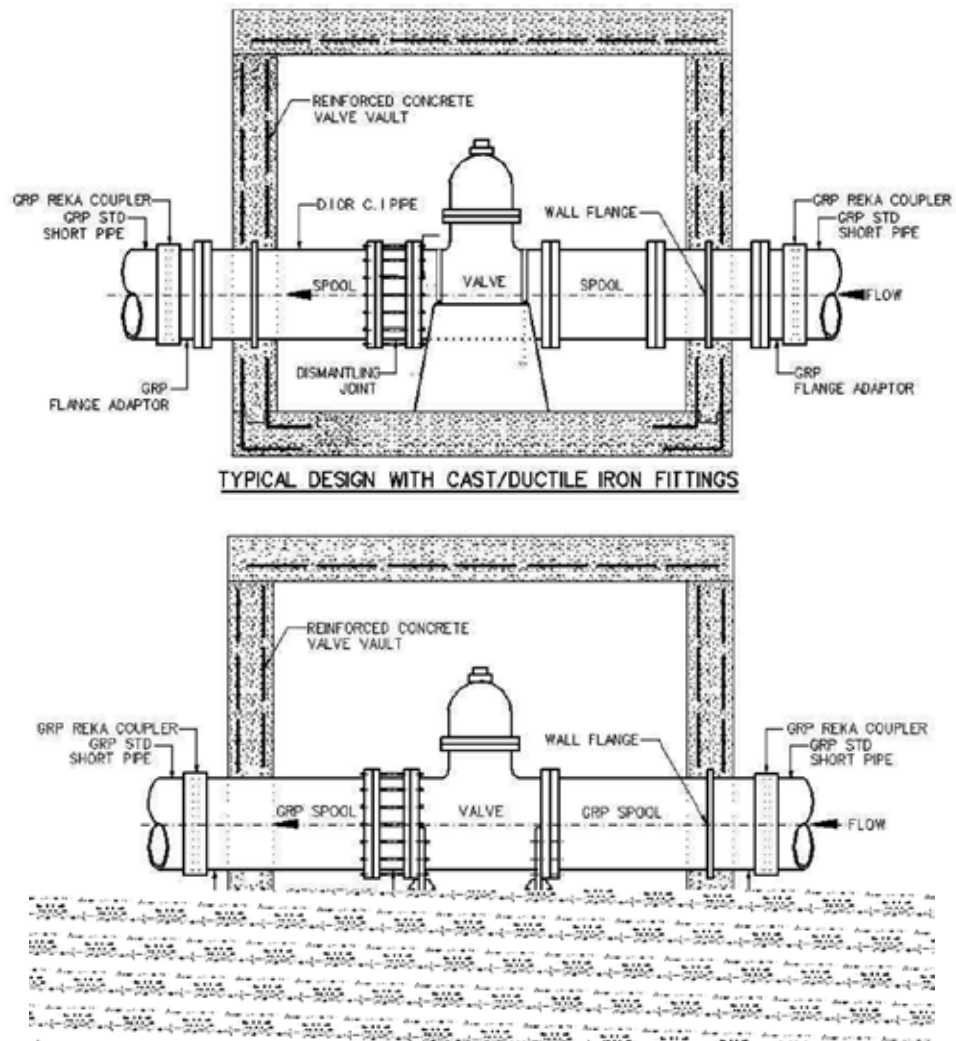
Figure 16: Valve Chamber
