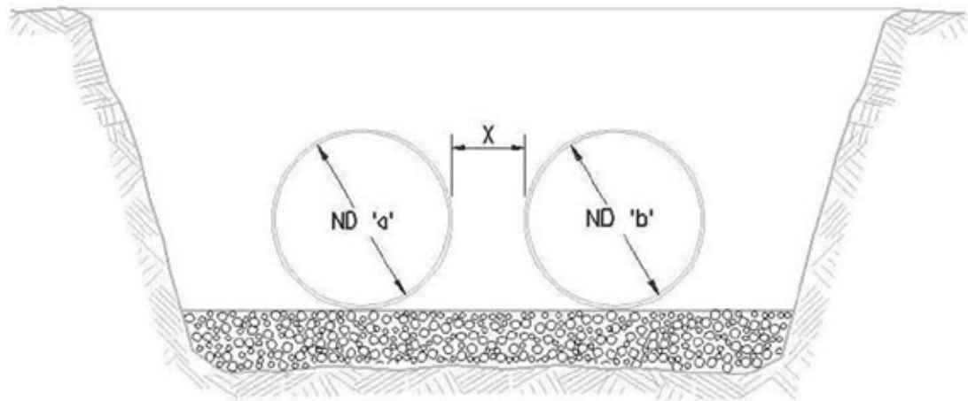
Figure 6: Pipes in the same trench
