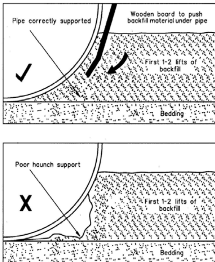
Figure 8: Backfilling pipe haunches
